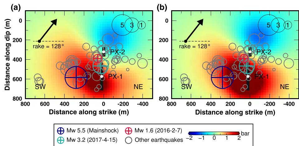
Figure 9. Total Coulomb stress change ( \Delta CFS ) on the fault plane caused by injection at the wells PX-1 and PX-2. (a) \Delta CFS without an impermeable core. This is the sum of the values of \Delta CFS by PX-1 (Figure 8a) and PX-2 (Figure 8e). (b) \Delta CFS with the impermeable core. Thickness and hydraulic diffusivity, D , of the core are 10 m and 10^{-6} \text{ m}^2/\text{s} , respectively, the same as those of Ellsworth et al. (2019) and KGC (2019; Figure 4b). See Figure S7 for pore pressure change, shear stress, and normal stress changes by PX-1 and PX-2. Only the earthquakes associated with the injection at PX-2 are plotted (Woo et al., 2019). No temporal Gaussian filter is applied. Information of the fault geometry and earthquake locations are taken from KGC (2019) and Woo et al. (2019).
